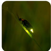
firefly
